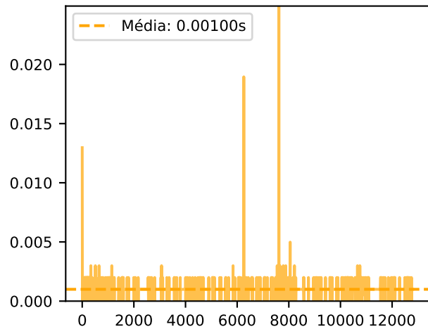
Recv \Delta t (local_time) | 1280Hz 5ch
