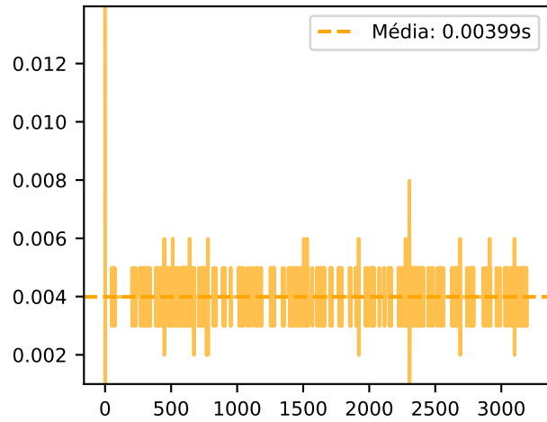
Recv \Delta t (local_time) | 1280Hz 5ch
