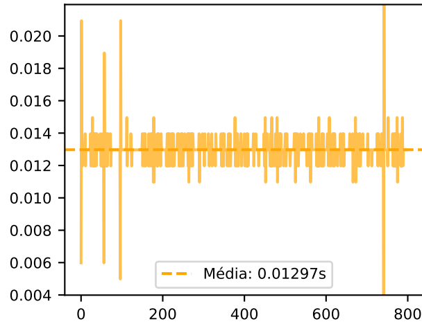
Recv \Delta t (local_time) | 320Hz 5ch
